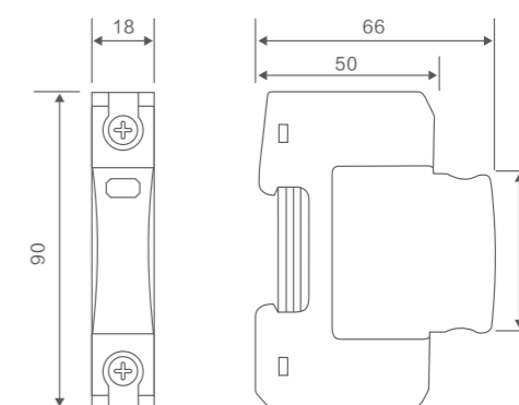
WR-T2T3-AC Dimension diagram
