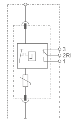
WR-T2T3-AC Basic circuit diagram
